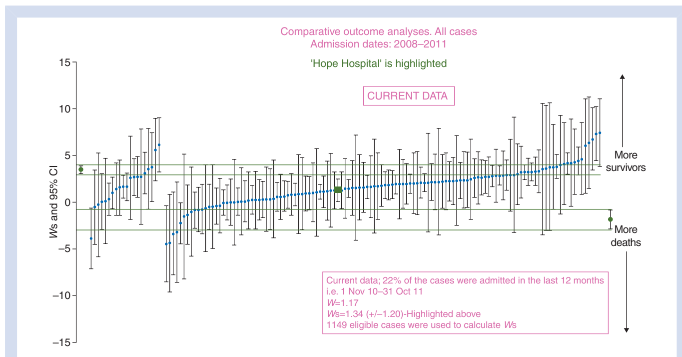
Fig 3 Example of hospital observed – expected mortality rates using caterpillar plot from the TARN. (The first author’s hospital is highlighted in an excerpt from the TARN ‘Hope Hospital quarterly report 2008–2011’.)
